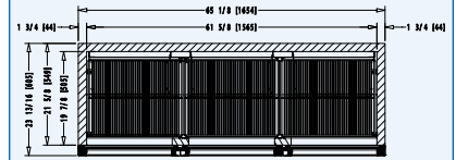
Top view / Vista superior: In [mm] / Pulg. [mm]:
