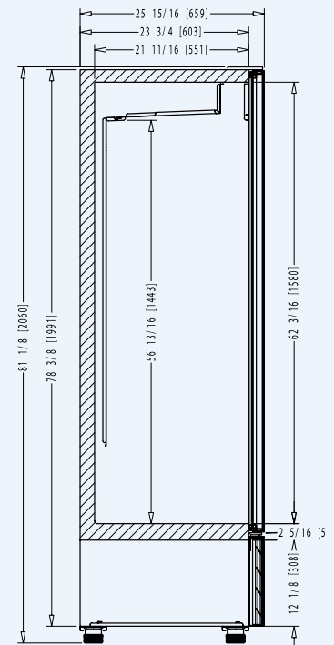
Side view / Vista lateral: In [mm] / Pulg. [mm]:
