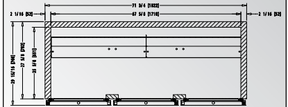
Top view / Vista superior: In [mm] / Pulg. [mm]:
