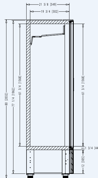
Side view / Vista lateral: In [mm] / Pulg. [mm]:
