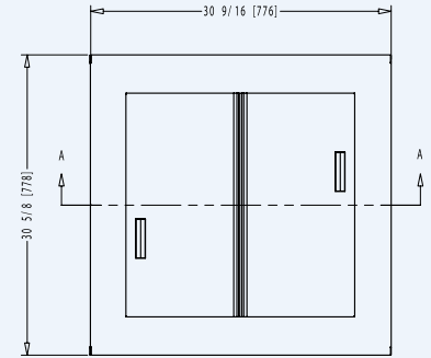
Top view / Vista superior: In [mm] / Pulg. [mm]:
